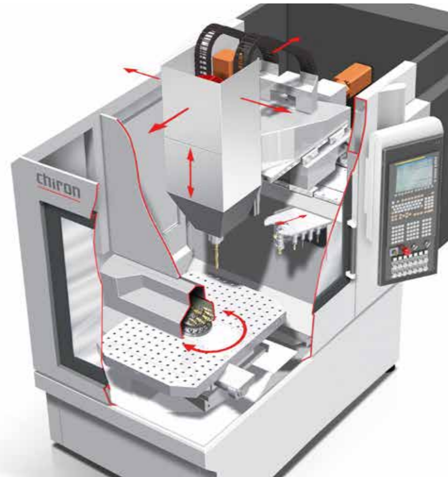
FZ 08 W: Compact and fast single-spindle machining center with integrated workpiece changing device 0°/180° for easy loading and unloading during machining.
