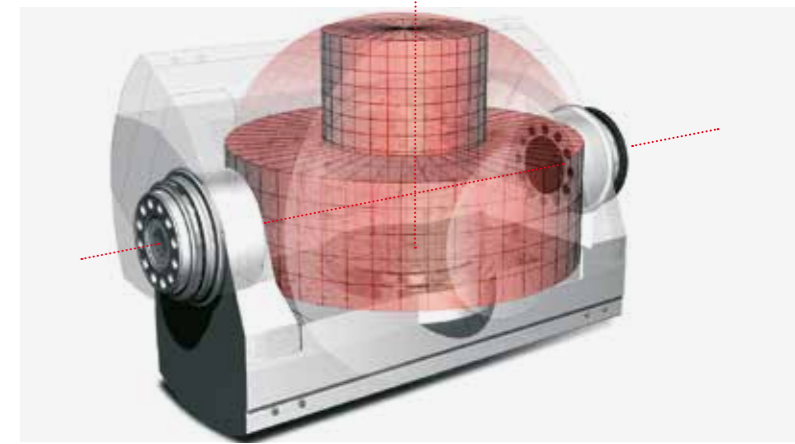
FZ 12 S five axis: Integrated CHIRON 2-axis rotary table, maintenancefree TORQUE drive technology and automatic tool change using the pick-up method.
