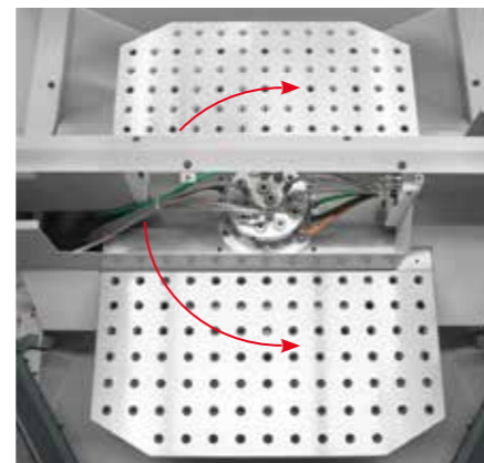
Workpiece changing device 0° / 180° with ample space for devices and NC rotary tables, such as the installation of a workpiece swivel device as the fourth NC-axis.
