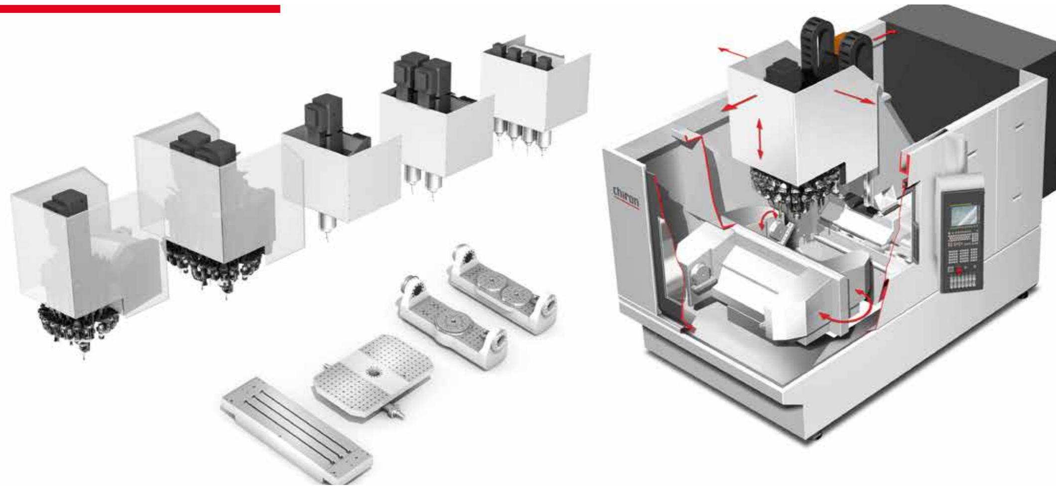
FZ 15 W: Compact, fast single-spindle machining center with integrated basket tool changer and integrated workpiece changing device 0°/180° for easy loading and unloading during machining.
